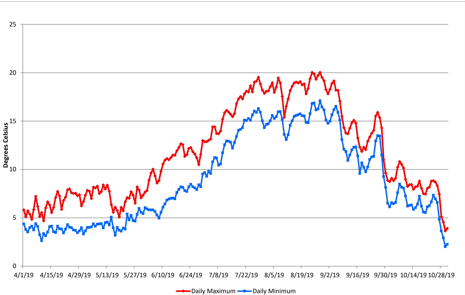
Figure 17. Daily Maximum and Minimum Water Temperatures in the SFAR above Kyburz Diversion, T26
