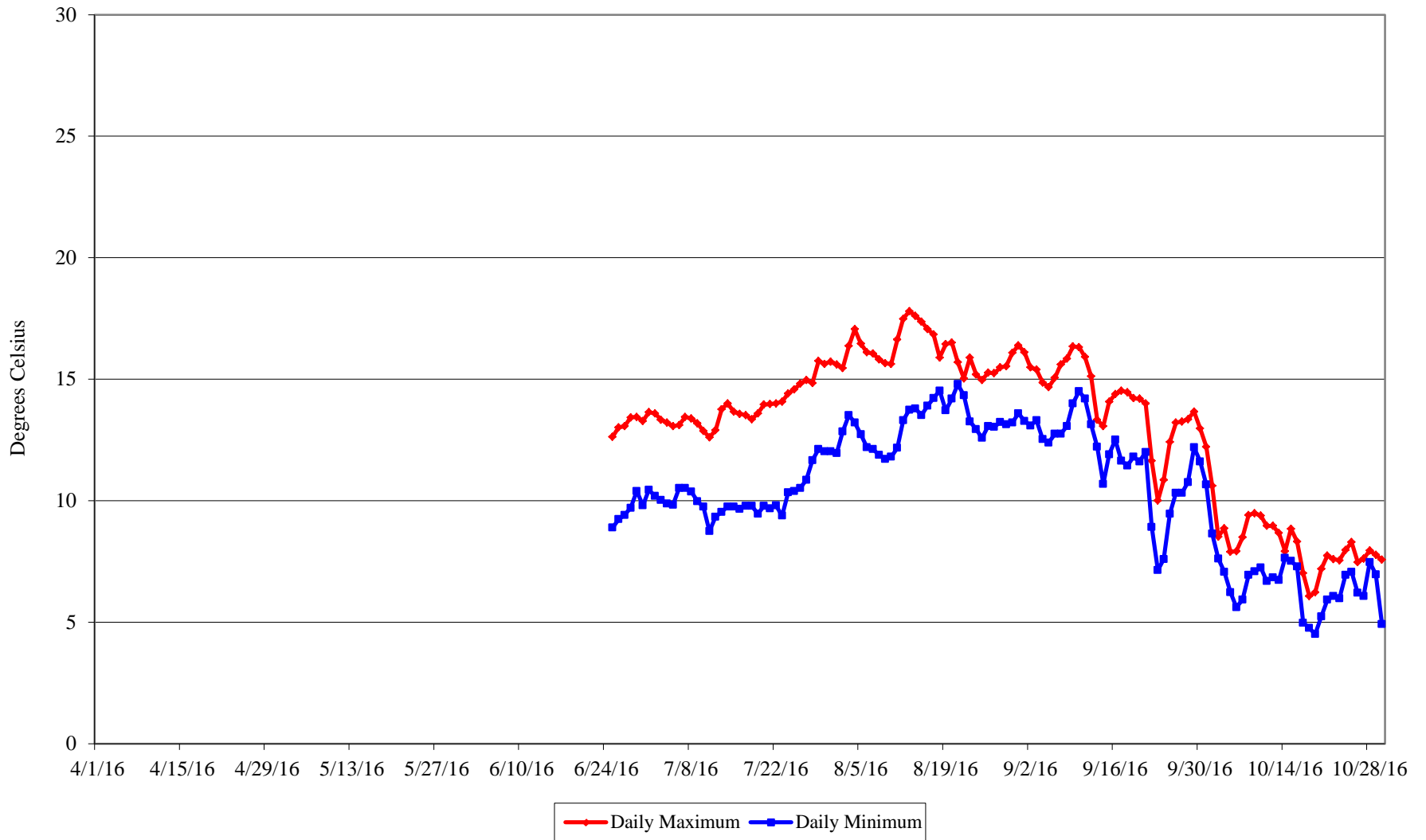
Figure 16. Daily Maximum and Minimum Water Temperatures Caples Creek upstream of the confluence with Silver Fork American River, T31
